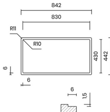
Lắp chìm Flushmount
